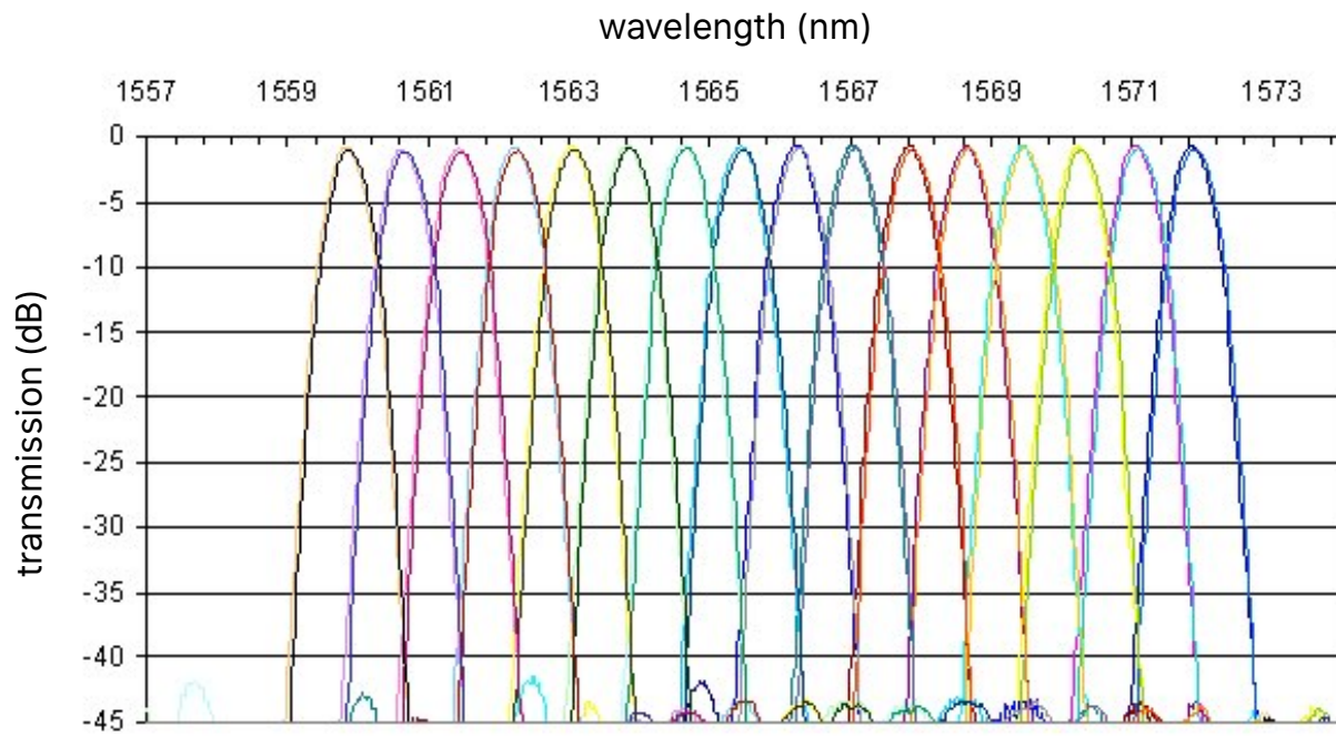
AAWG MUX/DEMUX spectrum showing ultra low loss and isolation performance.
